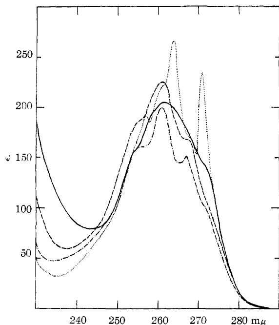
Fig. 1.—Representative ultraviolet absorption spectra in ethanol: o -di- t -butylbenzene (I), —; o - t -amylcumene (Vd), - - -; 1,1,4,4-tetramethyltetralin, . . . . .; \alpha,\alpha' - o -phenylene-diisobutyraldehyde hydrate (XIV), - . . . .
